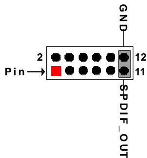
J1: Pin(11&12) SPDIF_OUT Head
