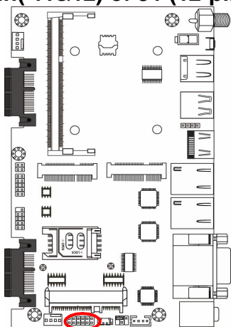
J1: Pin(11&12) SPDIF_OUT Head
