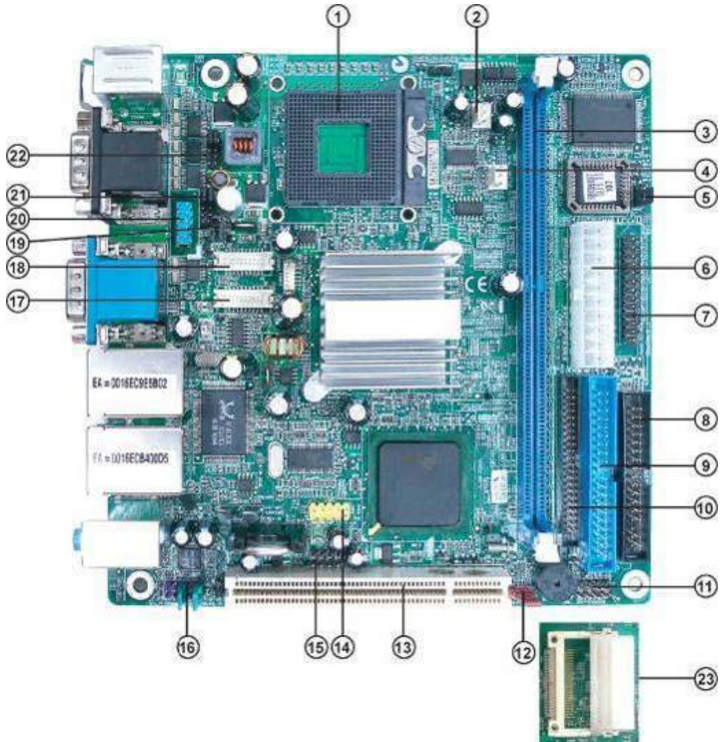
Figure 1.2: Mainboard Overview
